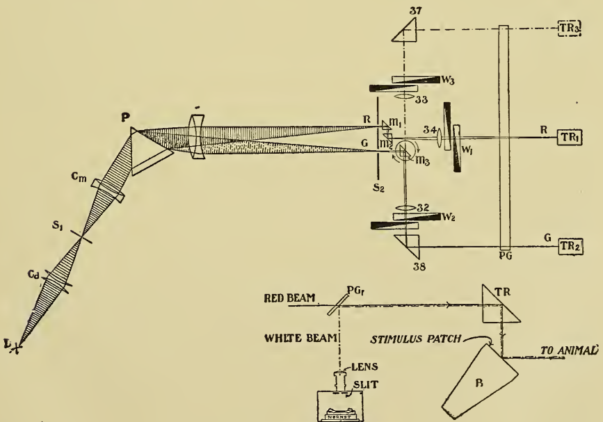
FIG. 3. GROUND PLAN OF MONOCHROMATIC LIGHT APPARATUS
